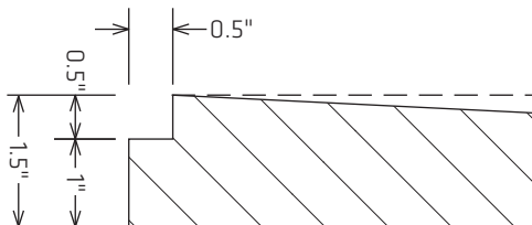
Detail 'Z' 5x
